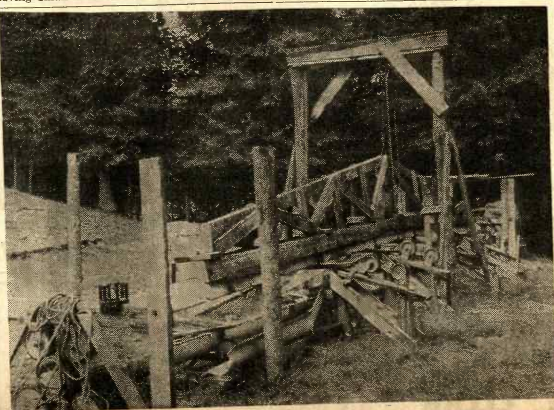
THIS MACHINE was used to make the pre-stressed, hollow concrete pole. The crude, work- ing model shown here, will be improved so that concrete poles can be made one every ten minutes.
